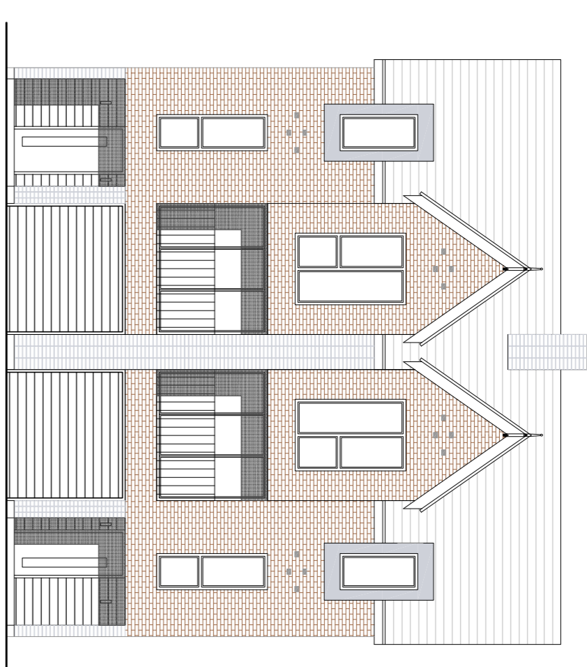
front elevation
