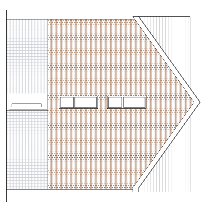
typical gable elevation
