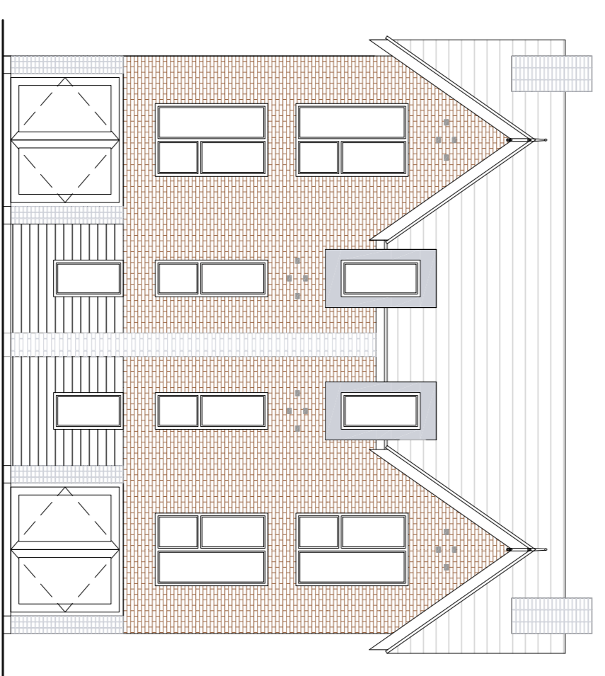
rear elevation
